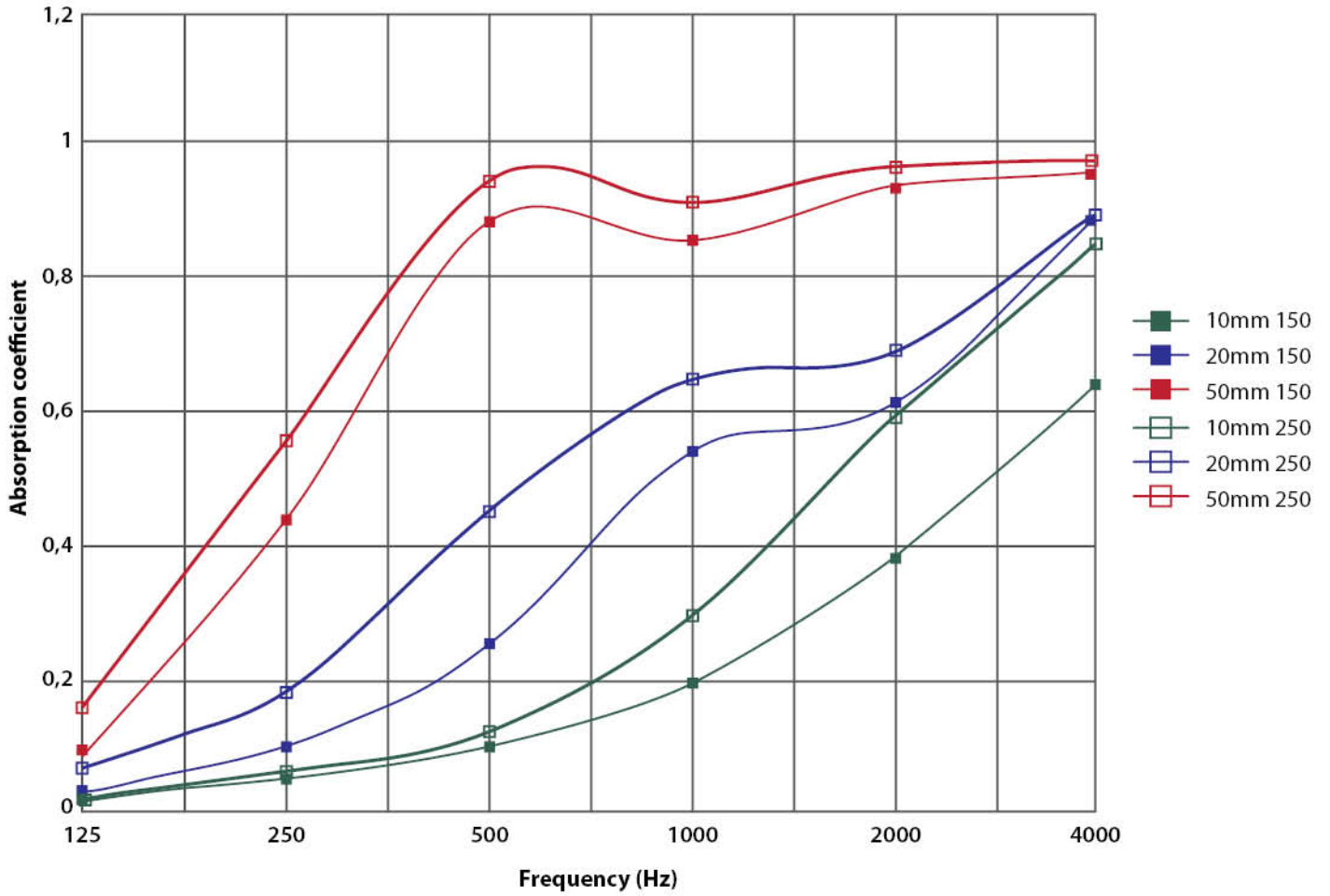
Absorption coefficient acc. to EN 354 for ISOSOUND
